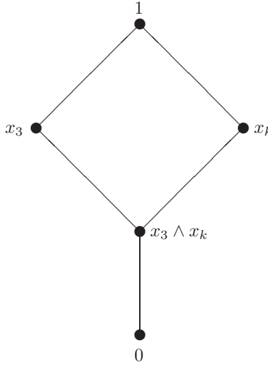
FIGURE 1. The lattice X_k , for k \in \{1, 2\}
